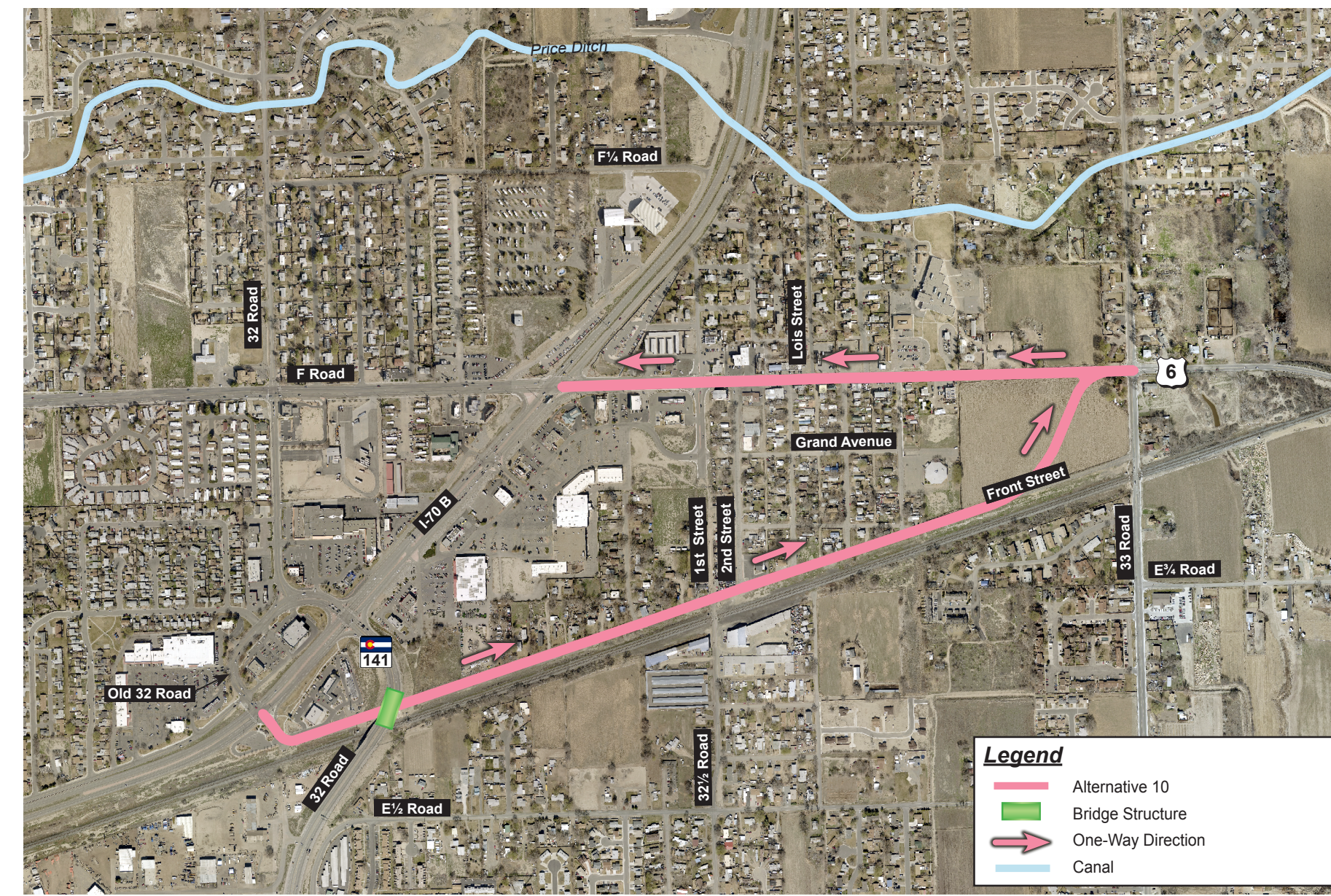
Alternative 10 - Front Street/US 6 One-Way Couplet, Old 32 Road to 33 Road
