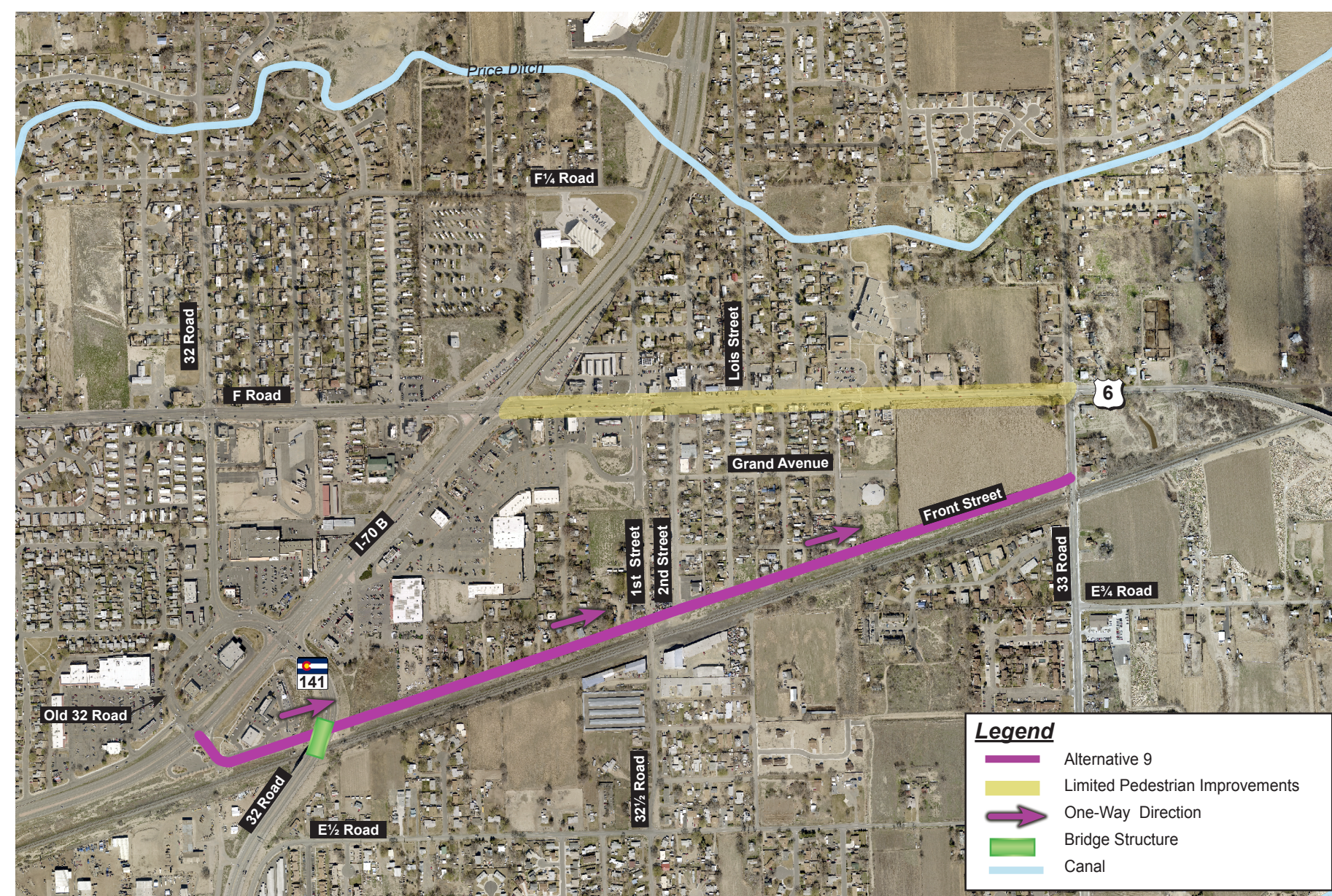
Alternative 9 - Front Street Connection One-Way Eastbound, Old 32 Road to 33 Road
