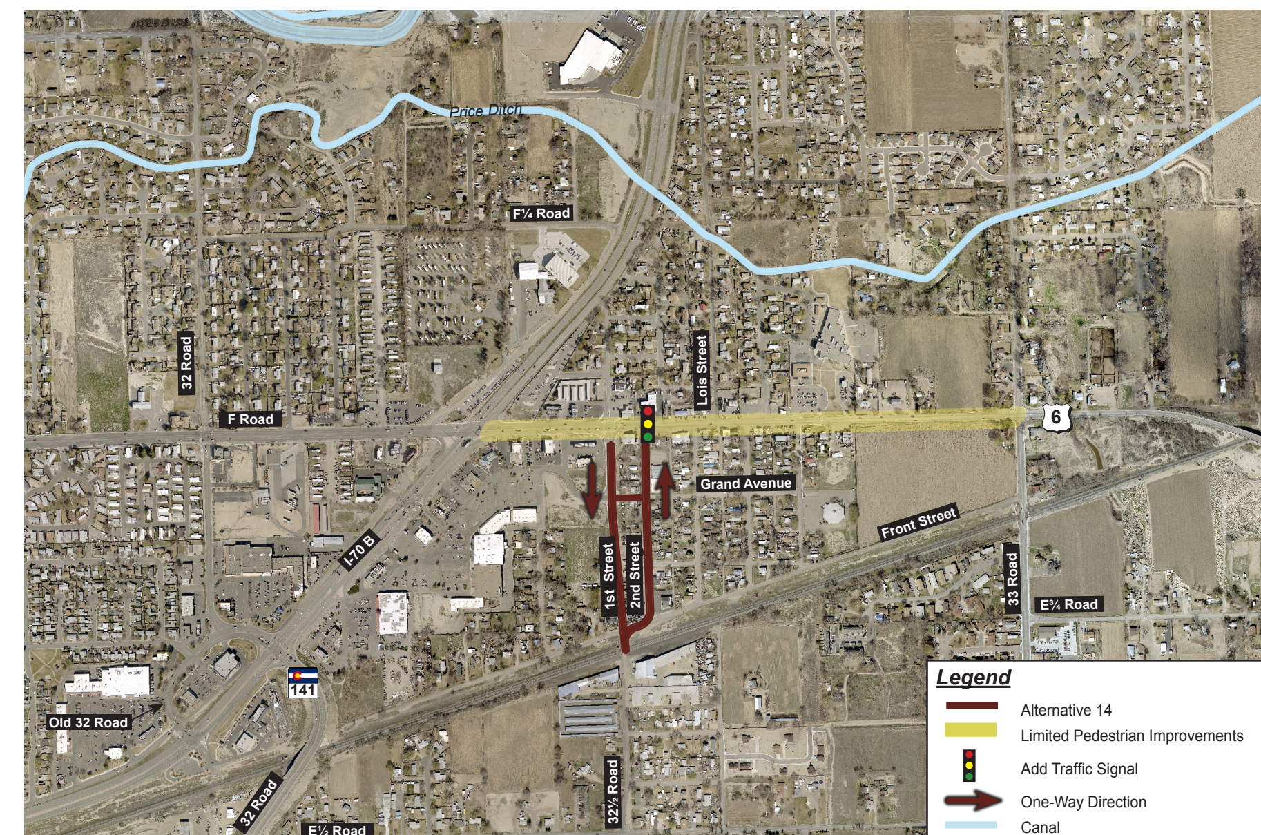
Alternative 14 - 1st/2nd Street One-Way Couplet
