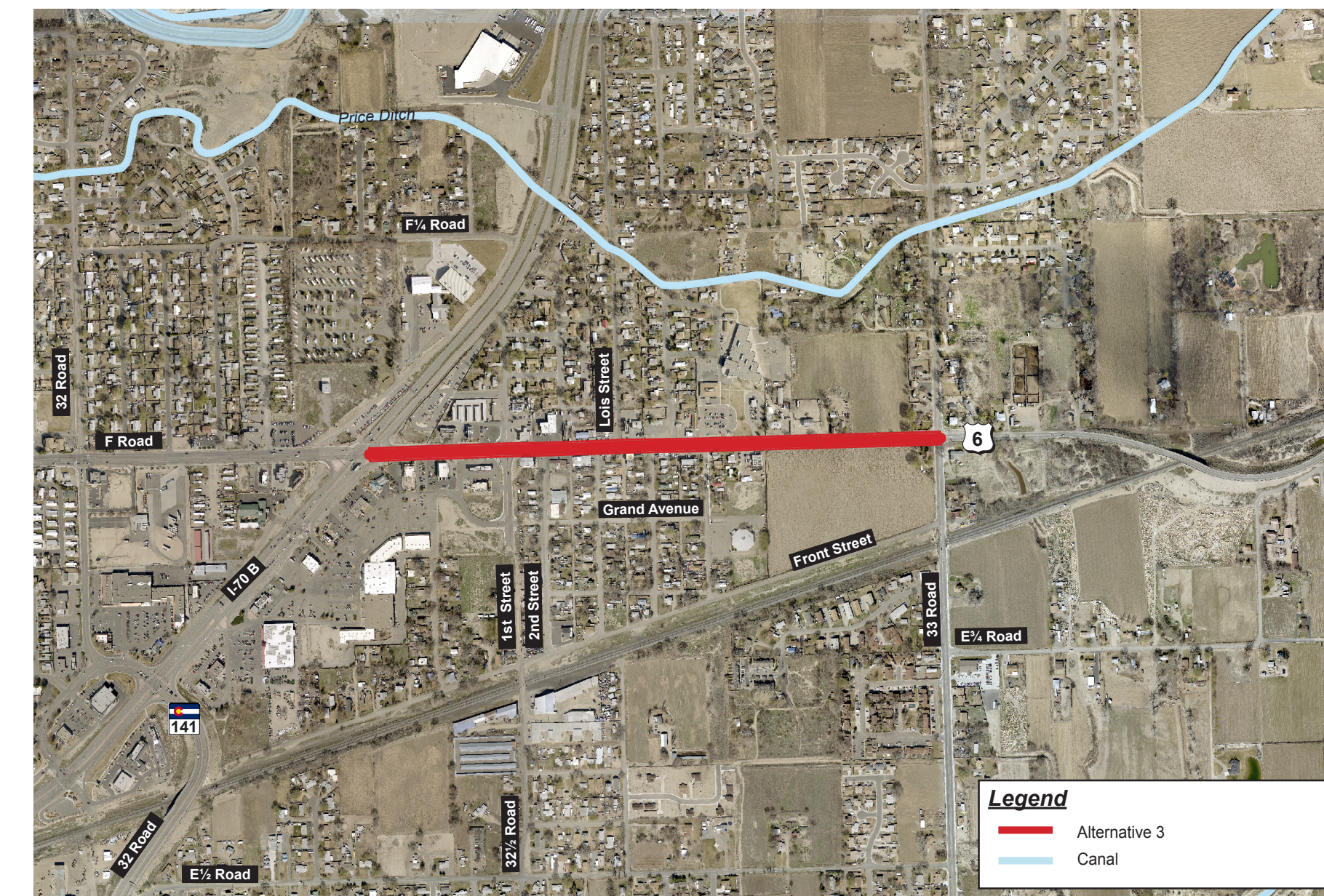
Alternative 3 - US 6 Four Through Lanes
